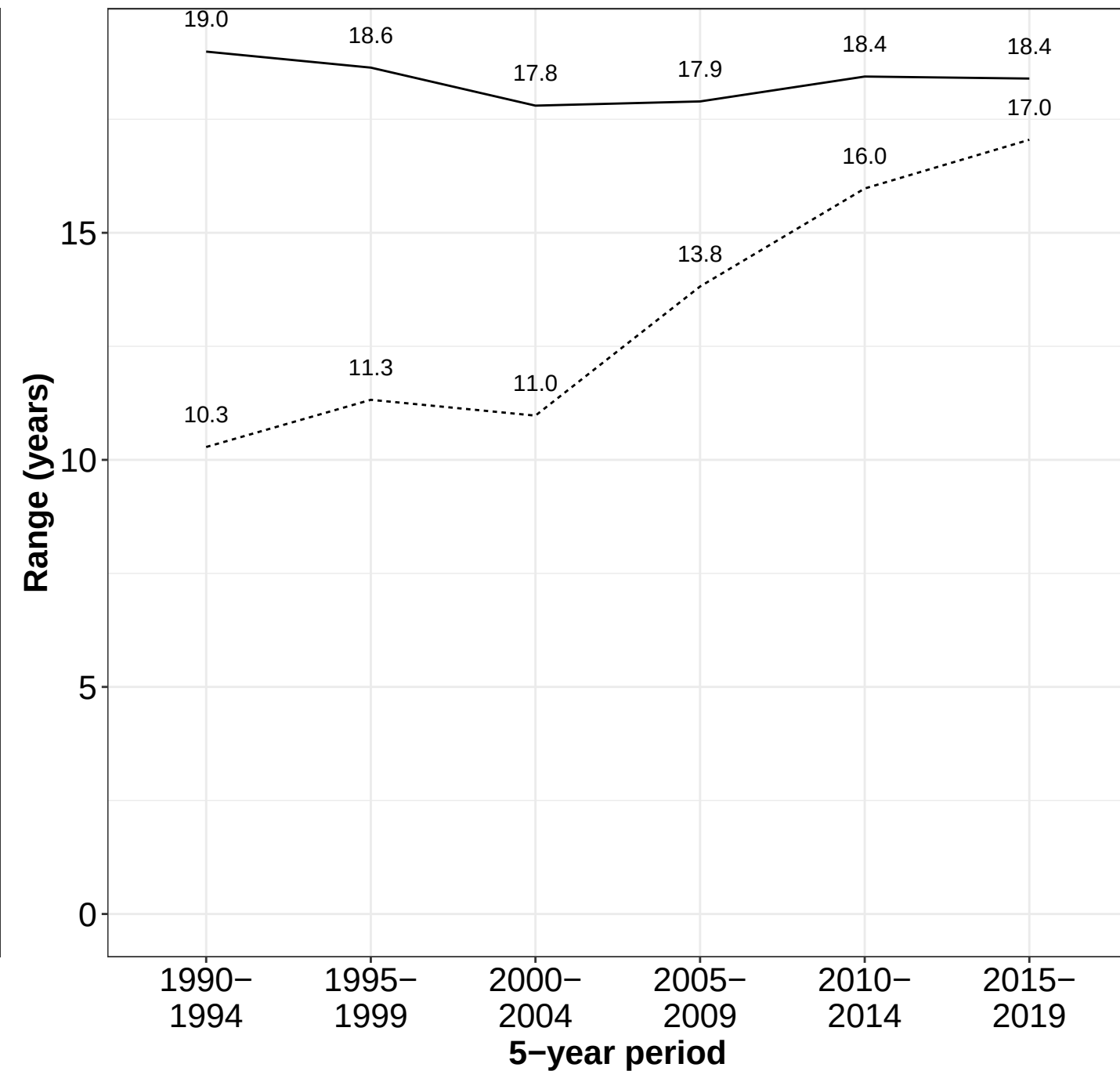
Range (maximum-minimum)
